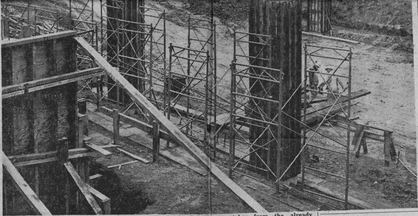
Concrete piers are being erected to support the freeway bridge over the Park avenue
