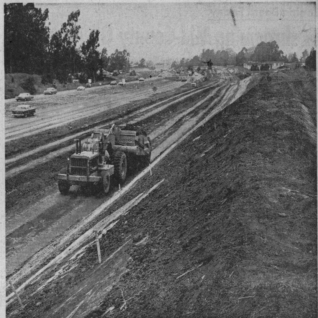
This heavily burdened carry-all needs additional propulsion from two caterpillars in order to move its load of dirt along the frontage road north of the Santa Cruz-Watsonville freeway. ♦ ♦ ♦
